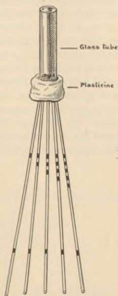
FIG. 125.—WRIGHT'S MANY STEMMED PIPET.
