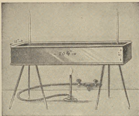
FIG. 138.—A VERY SIMPLE AND EFFICIENT WATER-BATH USED BY THE AUTHOR FOR THE INACTIVATION OF SERA AND FOR SECONDARY INCUBATION. Size is indicated. (Amer. Jour. Syphilis 1922, 6, 92.)
