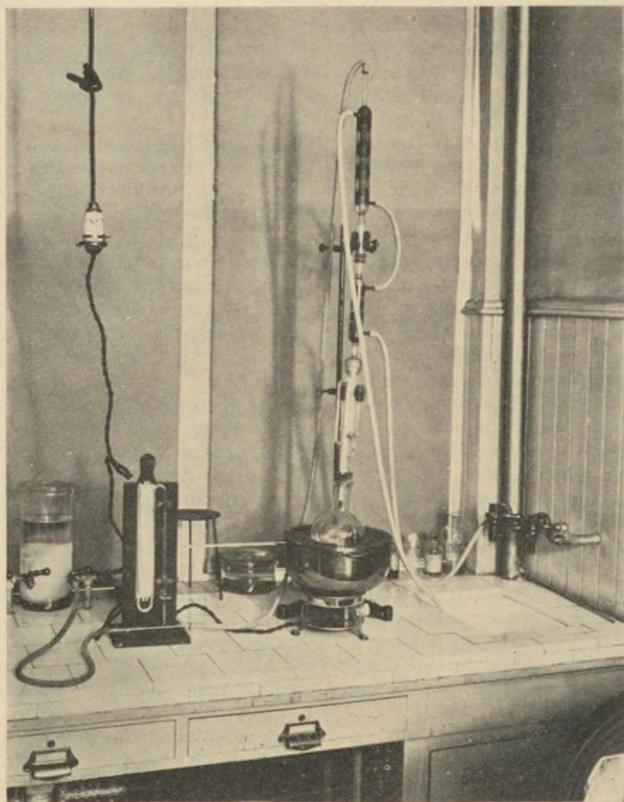
FIG. 145.—A SOXHLET EXTRACTION APPARATUS WITH VACUUM.
