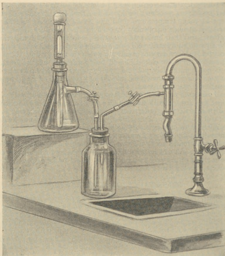
FIG. 49.—A SMALL BERKEFELD FILTER.
