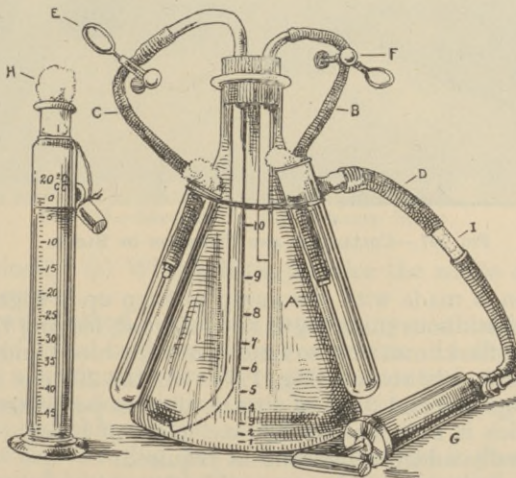
FIG. 196.—APPARATUS EMPLOYED BY THE AUTHOR FOR THE COLLECTION, CITRATING, AND INFUSION OF BLOOD.
