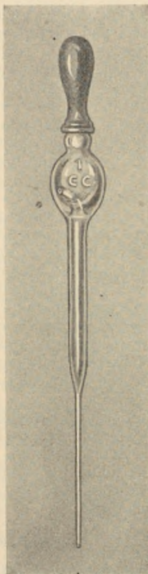
FIG. 86.—COMER'S AUTOMATIC PIPET. (Steele Glass Co., Philadelphia.)
