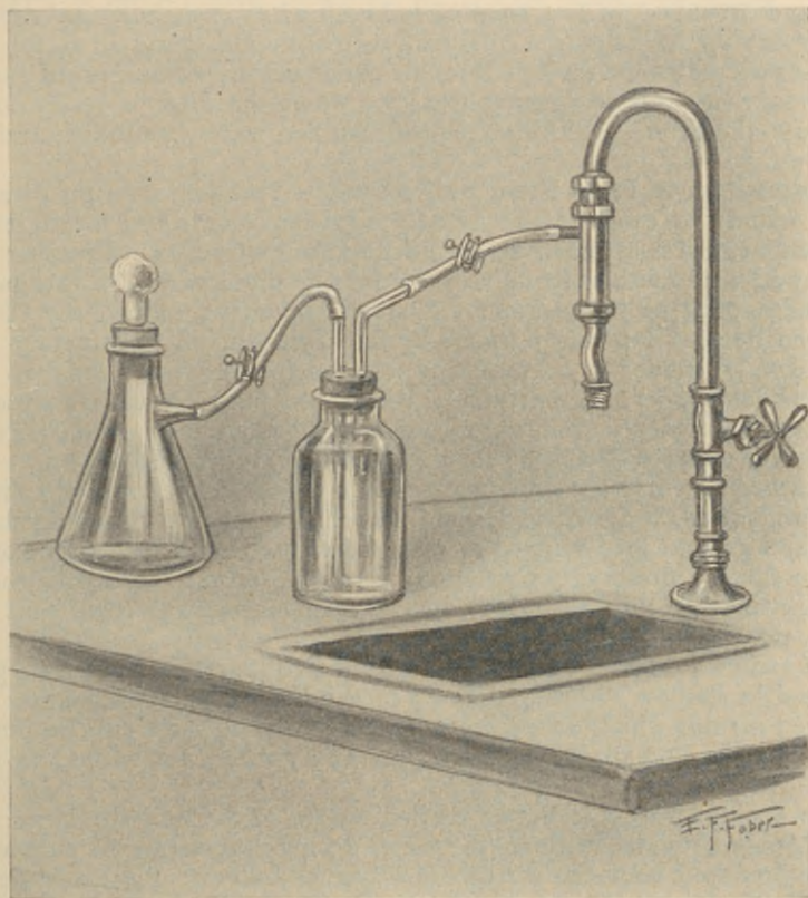
FIG. 50.—A FILTER.
